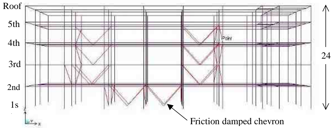
Figure 4. Block D, 3-dimensional analytical model of building, front view
