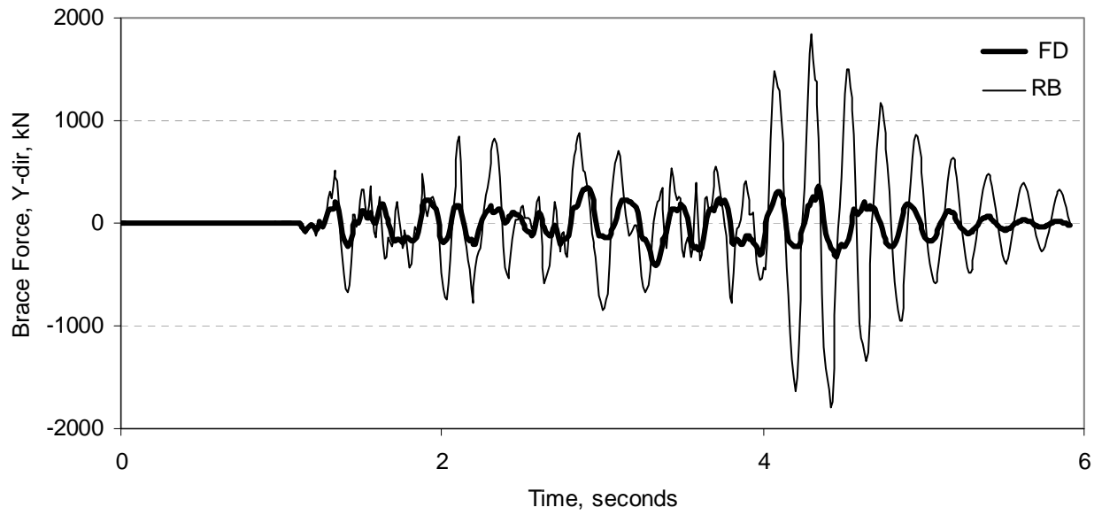
Figure 7. Time history of axial forces in 4 th floor single diagonal brace
