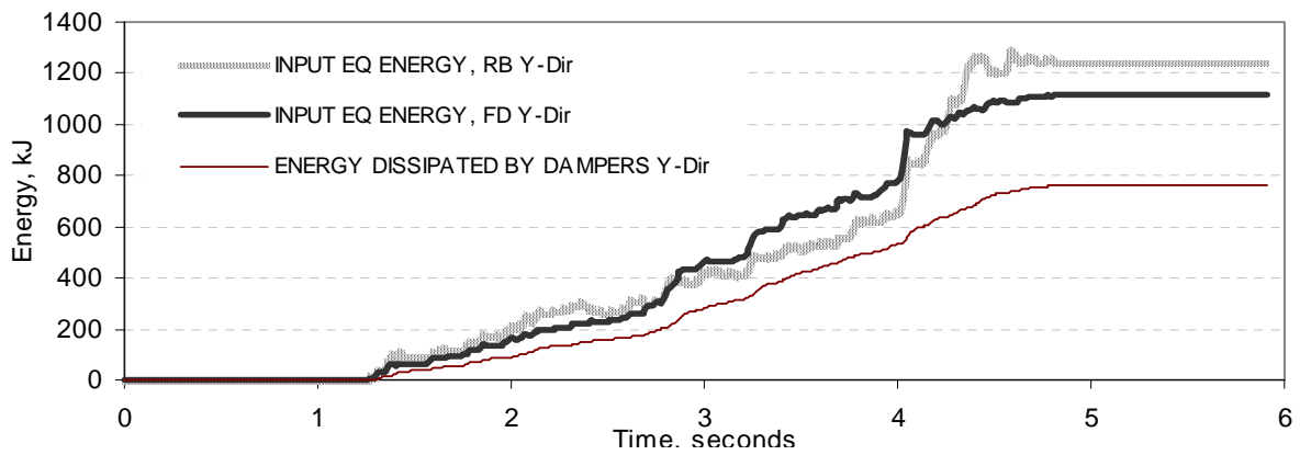
Figure 10. Time histories of energy input and energy dissipated
