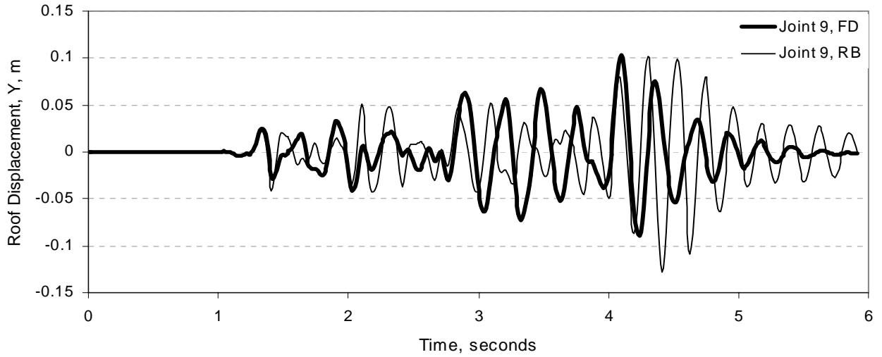
Figure 8. Time history of roof displacement
