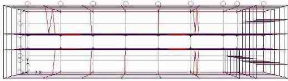
Figure 3. Block D, 3-dimensional analytical model of building, view from top down
