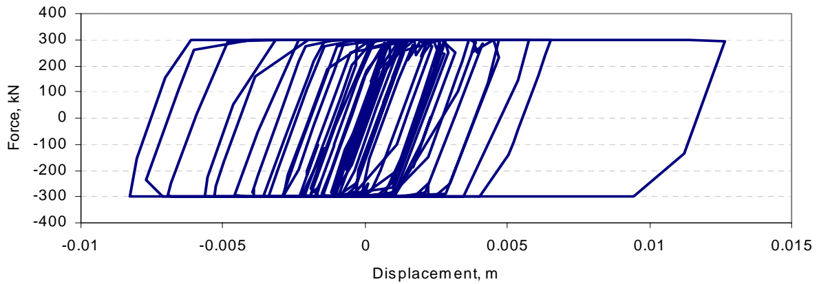
Figure 9. Hysteretic loop of friction damper
