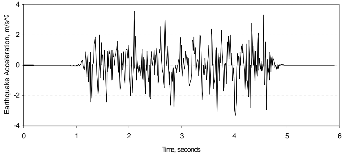
Figure 6. Time history of earthquake record
