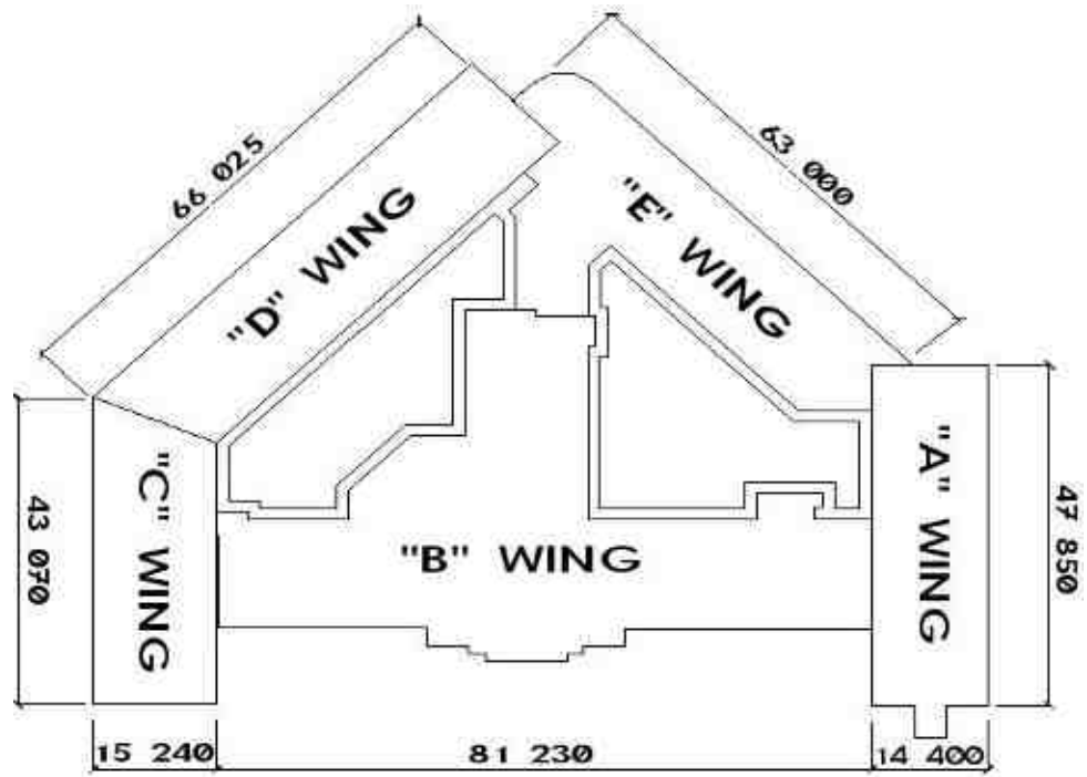
Figure 2. General layout plan of the hospital
